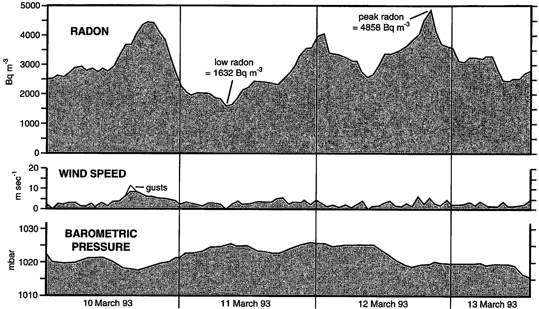
Figure 1. Indoor radon concentrations measured over the 3 1/2 days preceding the installation of a sub-slab depressurization radon reduction system in House B. Radon concentrations in the basement of House B were recorded hourly in the basement of House B beginning at 0100 hours on 10 March 1993, and ending at 1400 hours on 13 March 1993. Wind speed and barometric pressure, as measured at Reno-Cannon International Airport, were recorded hourly at about the same times that the radon measurements were recorded. Short-term gust speed is superimposed on the sustained wind speed curve.
