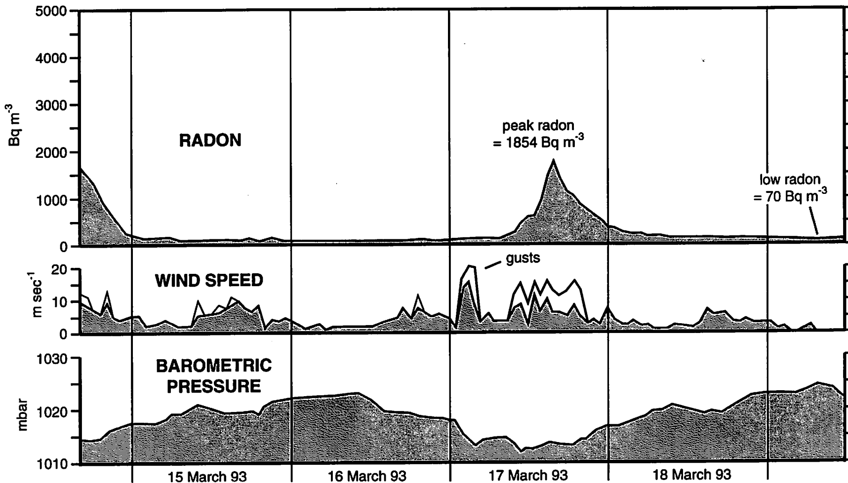
Figure 2. Indoor radon concentrations measured over the 5 days following the installation of a sub-slab depressurization radon reduction system in House B. Radon concentrations in the basement of House B were recorded hourly in the basement of House B beginning at 1600 hours on 14 March 1993, and ending at 1500 hours on 19 March 1993. Wind speed and barometric pressure, as measured at Reno-Cannon International Airport, were recorded hourly at about the same times that the radon measurements were recorded. Short-term gust speeds are superimposed on the sustained wind speed curve.
