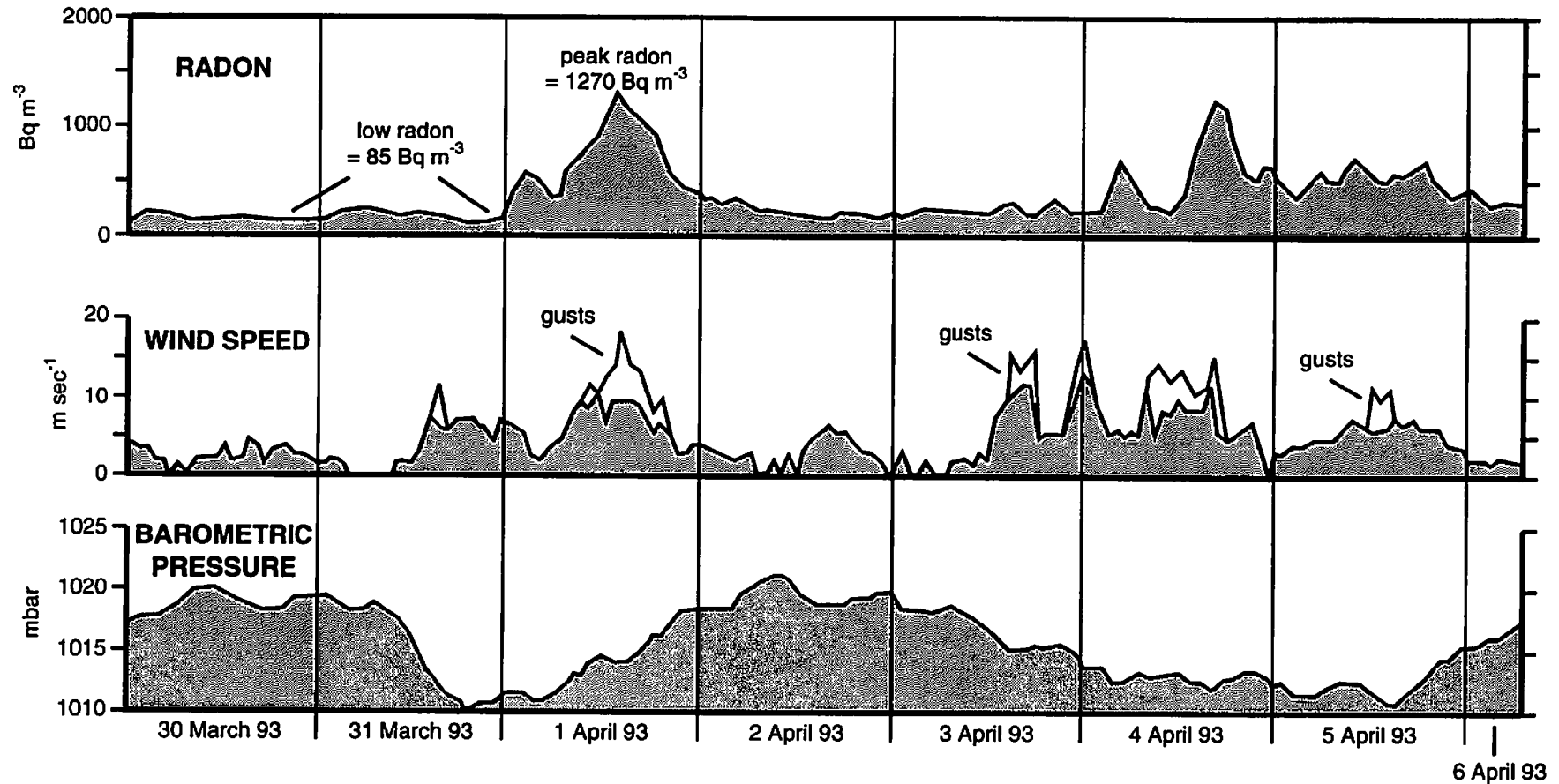
Figure 3. Indoor radon concentrations measured over approximately 7 days, a month after the installation of a sub-slab depressurization radon reduction system in House A. Radon concentrations in the basement of House A were recorded hourly beginning at 0100 hours on 30 March 1993, and ending at 0700 hours on 6 April 1993. Wind speed and barometric pressure, as measured at Reno-Cannon International Airport, were recorded hourly at about the same times that the radon measurements were recorded. Short-term gust speeds are superimposed on the sustained wind speed curve.
